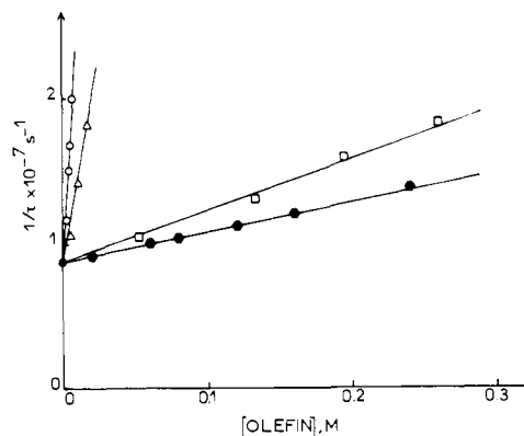
Figure 1. Plot of the pseudo-first-order rate constants for the growth of the ylide ( 1/\tau ) vs [olefin], at 25 °C in isoctane with [pyridine] = 0.45 mM: TME (○); HEX (●); ACN (□); CIACN (△).
